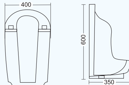
GI-408 | HALF STALL URINAL L 350 W 400 H 600mm
