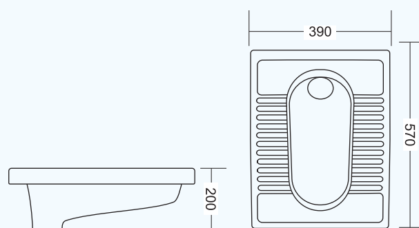
GI-422 ORISSA PAN (20") L 570 W 390 H 200mm
