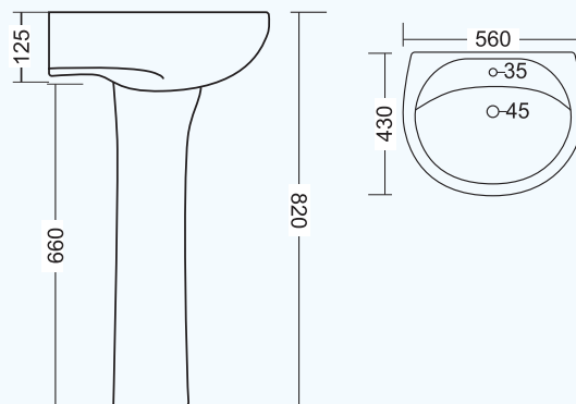
GI-501 22" x 16" REPOSE SET L 430 W 560 H 820mm
