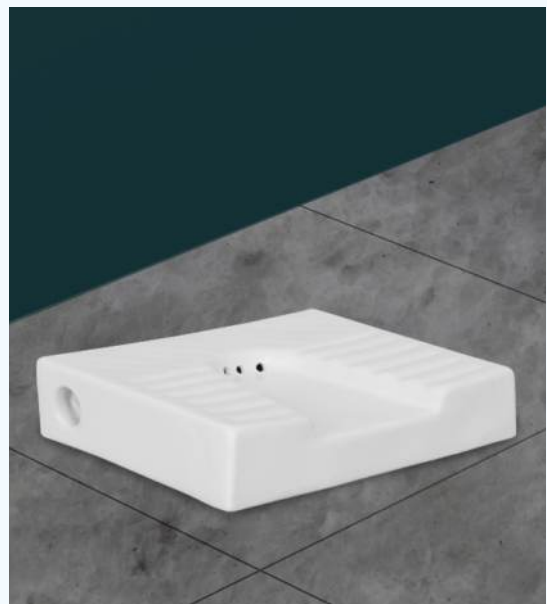
GI-410 | LADIES URINAL L 360 W 445 H 100mm
