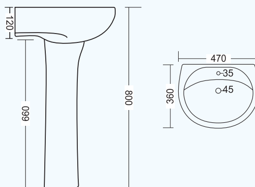
GI-502 18" x 14" MINI REPOSE SET L 360 W 470 H 800mm
