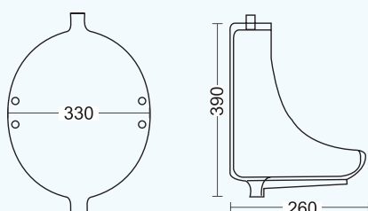
GI-409 | FLAT BACK URINAL L 260 W 330 H 390mm
