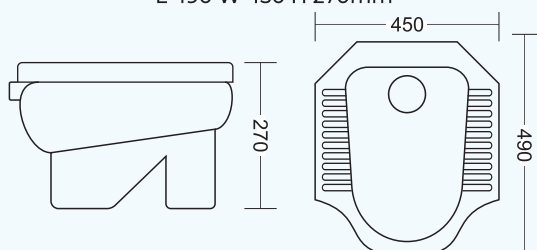
GI-432 | CHINA PAN
