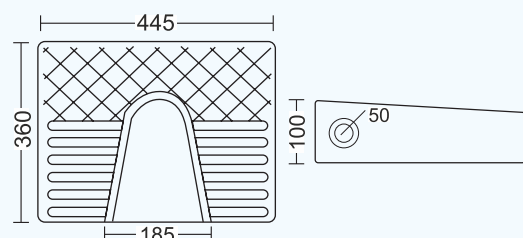
GI-410 | LADIES URINAL L 360 W 445 H 100mm
