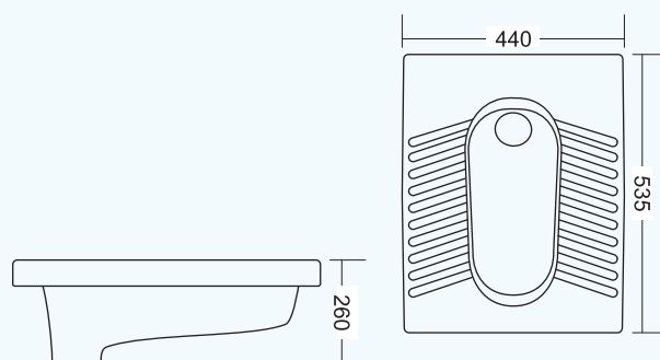
GI-421 DELUXE ORISSA PAN (20") L 535 W 440 H 260mm
