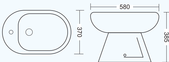
GI-407 | BIDET L 580 W 370 H 385mm
